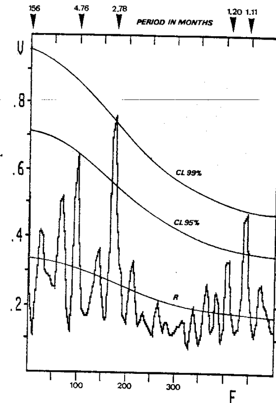
Figure 16: Blackman-Tukey power spectrum of flare-generated X-ray bursts equal to or greater than class X1 observed 1970 to 1982 by means of satellite instrumentation. The frequency f of investigated cycles is measured in millicycles per sampling interval of half a month. The ordinate axis represents the relative variance V of the respective frequencies. Periods of outstanding peaks, pointing to cycles of flares, are indicated on top of the figure. The significance of the deviation of prominent peaks from the Markov red noise ( R ) can be evaluated by means of the confidence level curves CL . The result provides evidence of cyclic features in the distribution of energetic solar flares.
