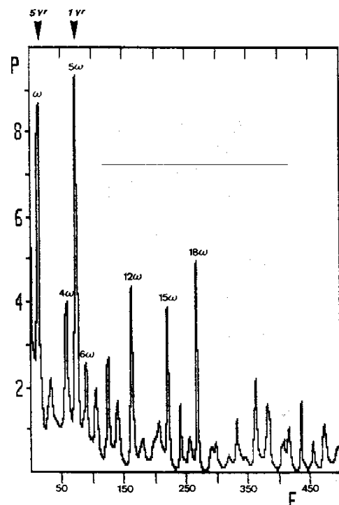
Figure 24: Maximum entropy spectrum of the running variance of the Sun's equatorial rotation rate (Mount Wilson data). The prominent peaks represent the mean period ( \omega ) of the JU-CM-CS cycles involved and its harmonics 4\omega , 5\omega , 6\omega , or simple multiples of these frequencies.
