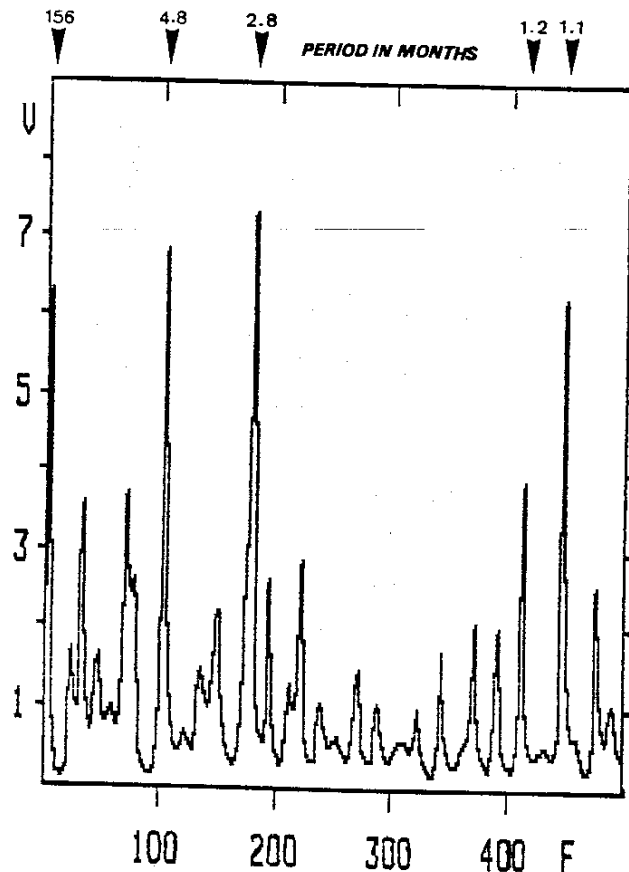
Figure 17: Maximum entropy spectrum of the same sample of X-ray bursts equal to or greater than class X1 as presented in Figure 16. The analysis based on the Burg-algorithm includes 312 data points and has a filter length of 82 coefficients. The frequency f is measured in millicycles per sampling interval of half a month. The ordinate axis indicates the relative variance of the respective frequencies. The outstanding peaks conform with those in the spectrum of Figure 16. This points to a cyclic pattern in the investigated sample of X-ray flares.
