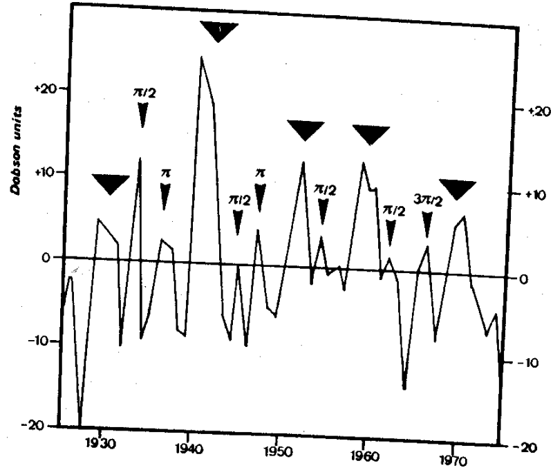
Figure 29: Arosa record of ozone levels since 1926 after H. U. Duetsch. The curve plots the deviation of annual mean values from the 50-year mean of 337 Dobson units. Triangles mark epochs of JU-CM-CS events. Arrow heads point to harmonics of cycles formed by consecutive Jupiter-CM conjunctions. The respective epochs meet peaks in the ozone column.
