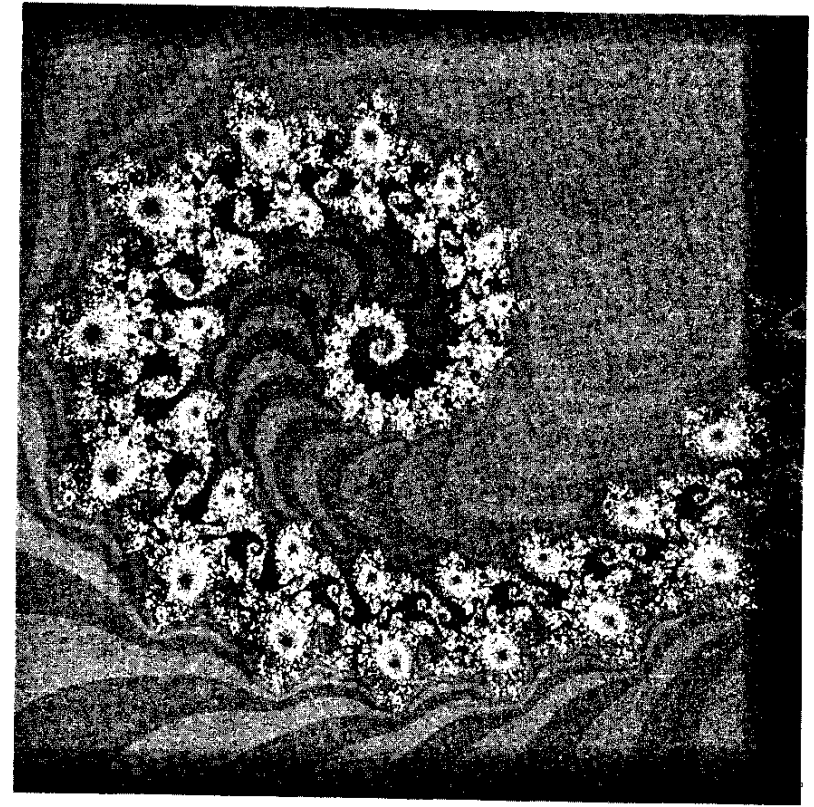
Figure 3: Boundary pattern, called Julia set, elaborated by H. O. Peitgen and P. H. Richter. Julia sets carry incredibly complex dynamics emerging from boundaries between domains of antagonistic attractors that compete for influence. In border regions with polar tension transition from one form of existence to another takes place: from order to disorder, magnetic to non-magnetic state, or however the opposite entities are to be interpreted that meet at the boundary.
