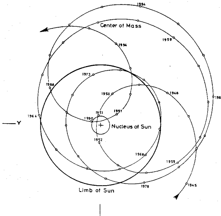
Figure 18: Position of the centre of mass of the solar system CM in the ecliptic plane relative to the Sun's centre CS for the years 1945 to 1995. Heliocentric representation and marking the limb of Sun make it easy to see whether CM is above or below the Sun's surface. The distance of both centres varies from 0.01 to 2.19 solar radii.
